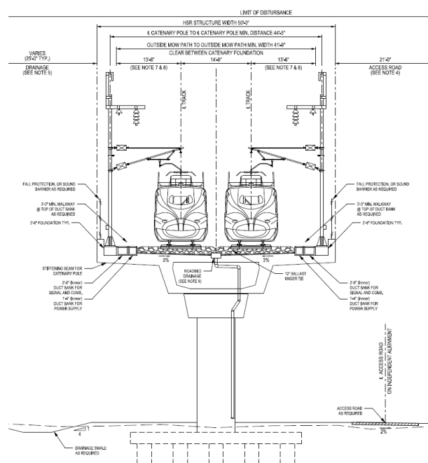
Fig.3- 8 Cross-sectional view of fully sealed dedicated tracks
